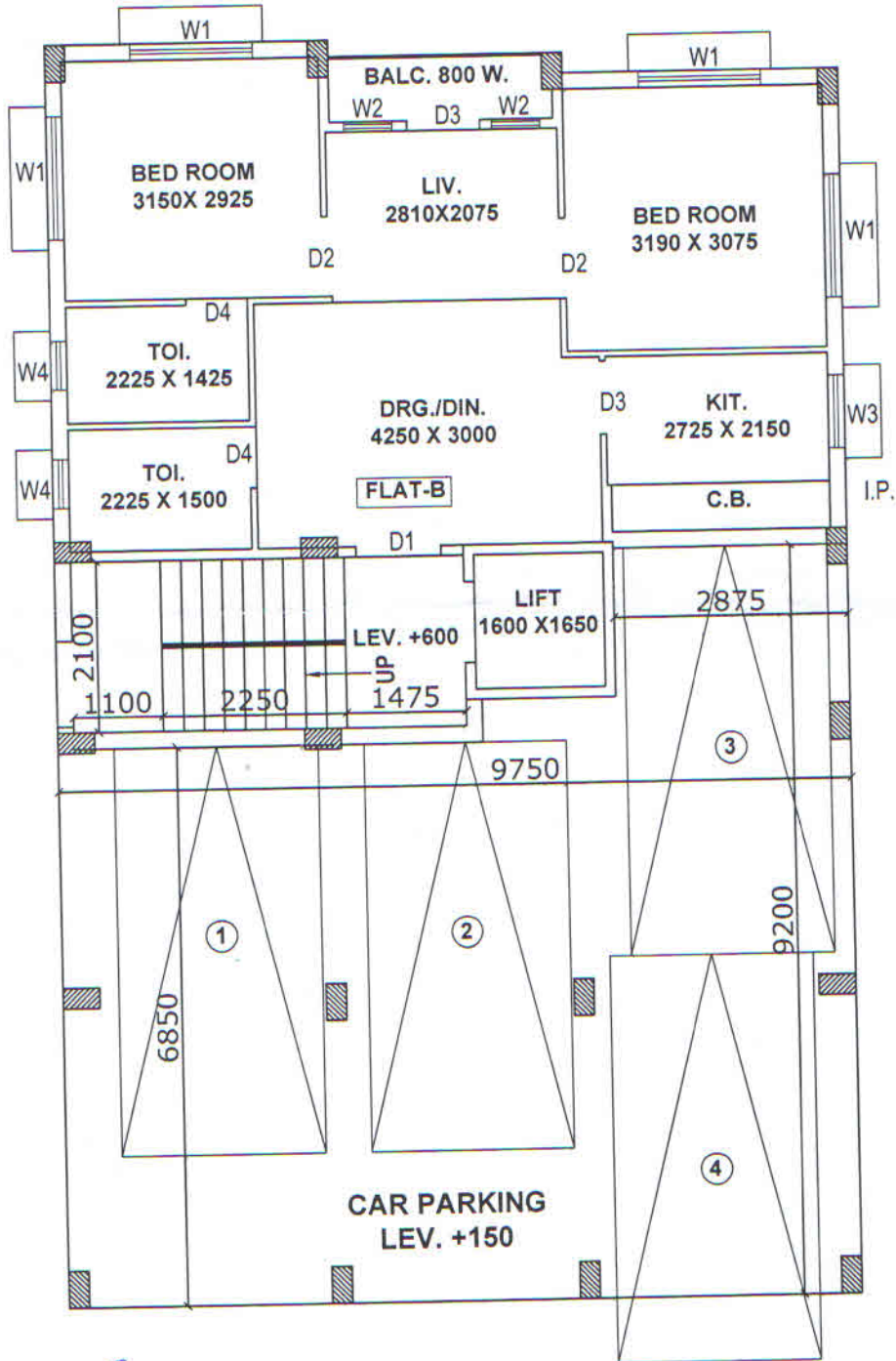
GROUND FLOOR PLAN 71, BAGUIATI 4TH. LANE.
