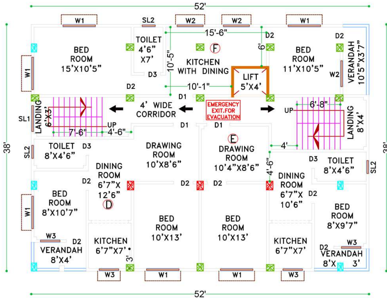
PROPOSED THIRD FLOOR PLAN SCALE:-1:96
