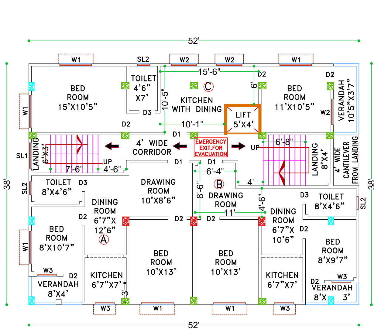
PROPOSED FIRST FLOOR PLAN SCALE: - 1:96
