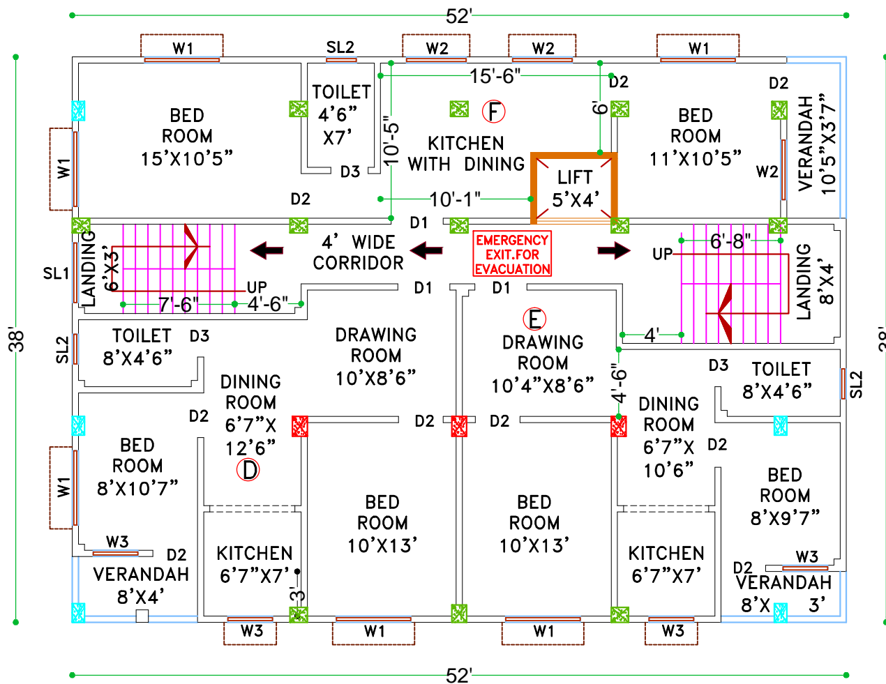
PROPOSED FOURTH FLOOR PLAN SCALE: - 1:96
