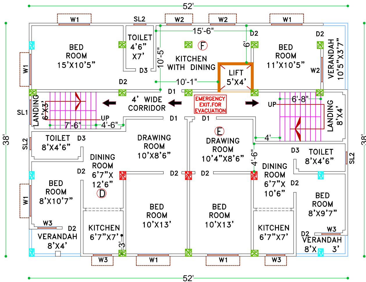
PROPOSED SECOND FLOOR PLAN SCALE: - 1:96
