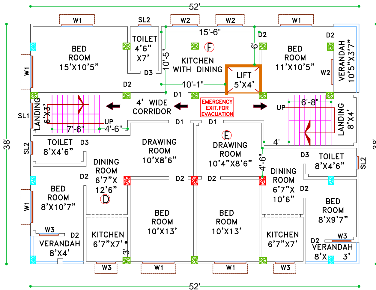
PROPOSED THIRD FLOOR PLAN SCALE: - 1:96
