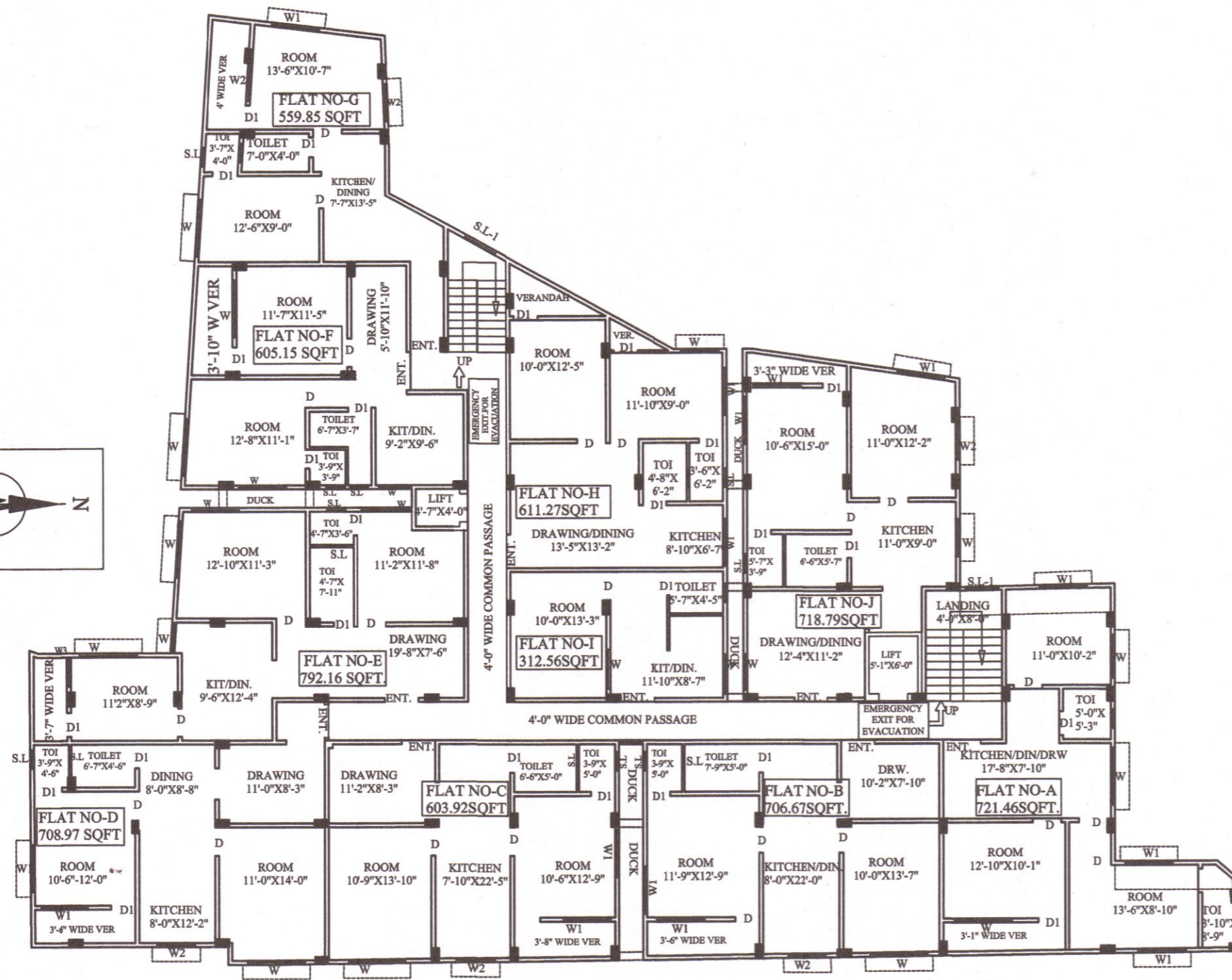
PROPOSED 2ND FLOOR PLAN SCALE 1:96
