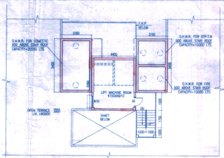
PART PLAN OF LIFT MACHINE ROOM BLOCK 1Q
