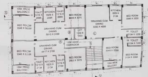
TYPICAL FLOOR PLAN (FIRST, SECOND & THIRD) SCALE - 1:100
