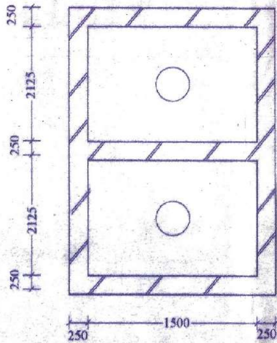
DETL. OF UNDER GROUND WATER RESERVIOR(U.G.R.)
