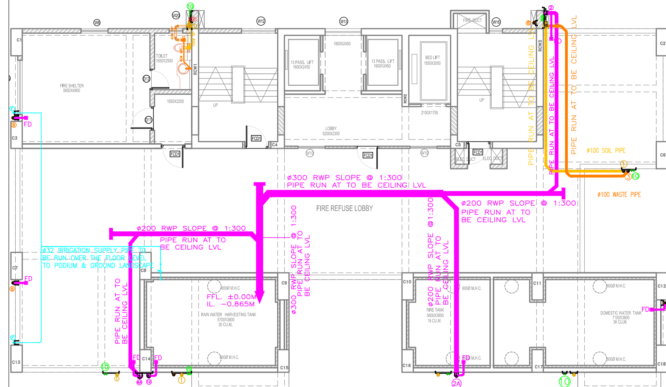
19TH FLOOR PLAN - DRAINAGE SCALE 1:75
