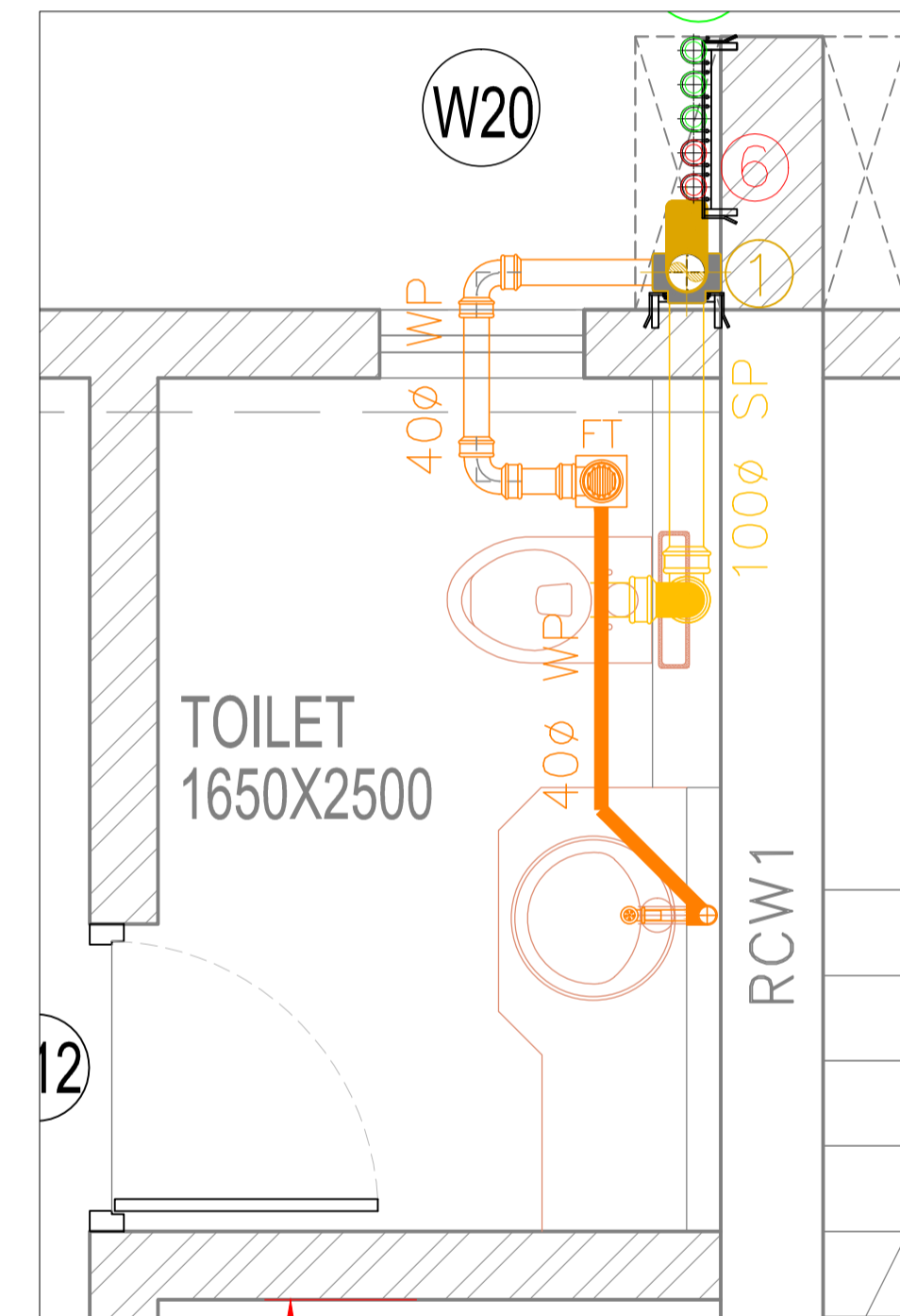
19TH FLOOR PLAN - TOILET DRAINAGE SCALE 1:20
