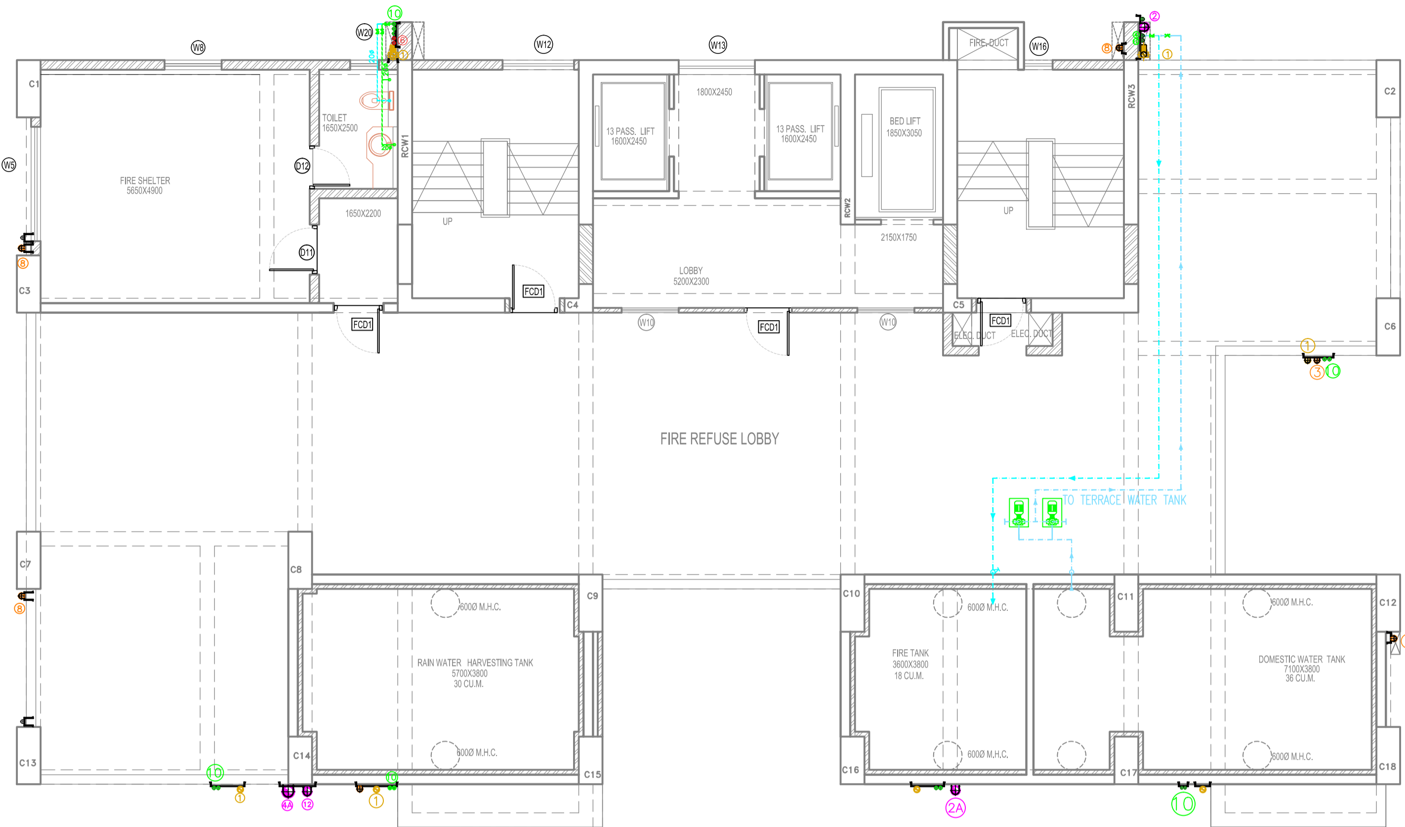
19TH FLOOR PLAN - WATER SUPPLY @ CLG. LVL SCALE 1:75
