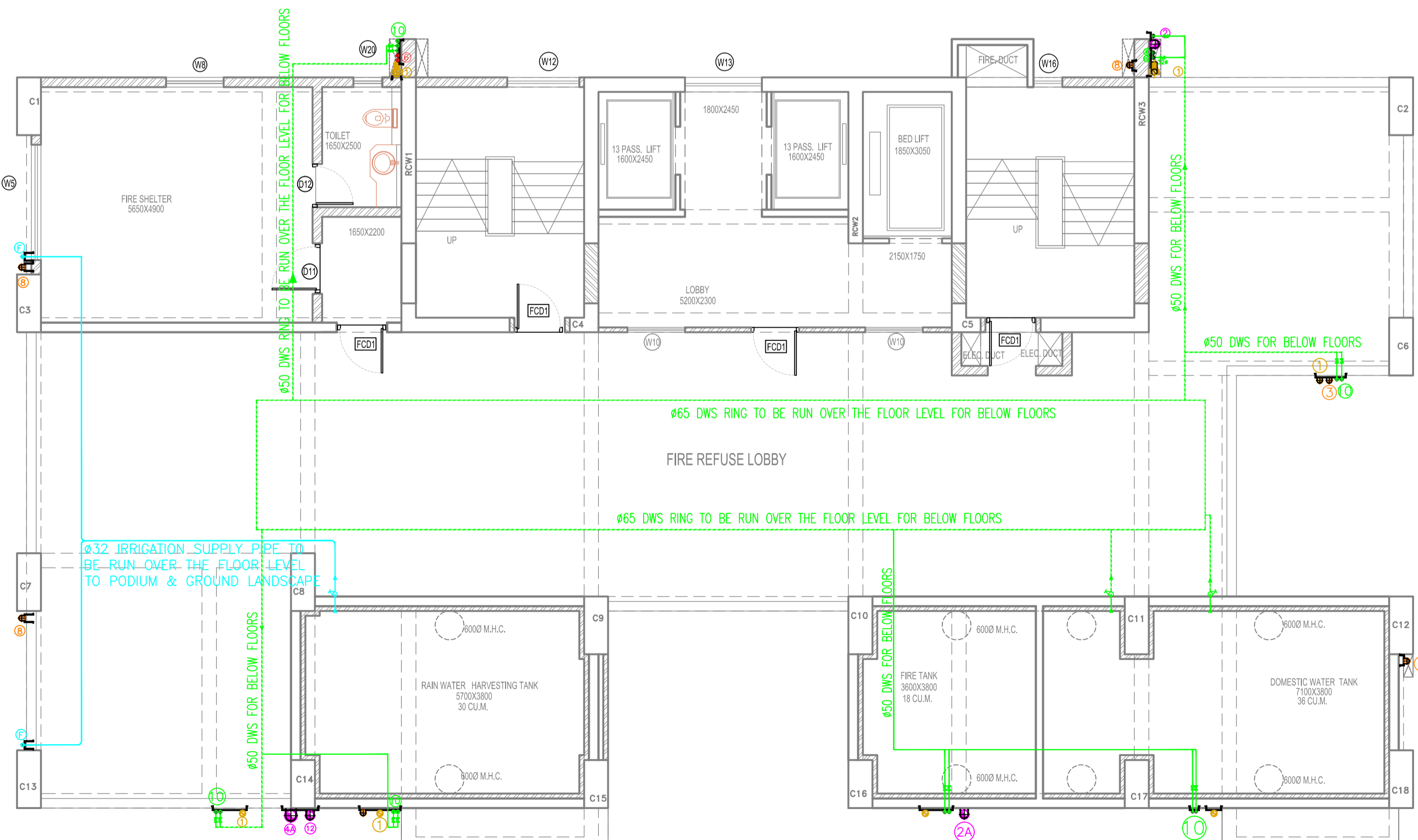
19TH FLOOR PLAN - WATER SUPPLY @ FLOOR LVL SCALE 1:75
