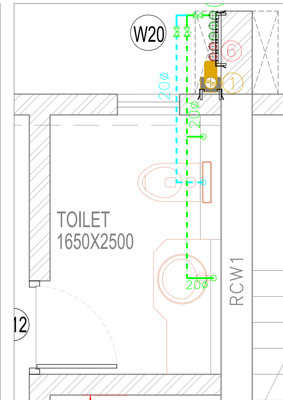
19TH FLOOR PLAN - TOILET WATER SUPPLY SCALE 1:20
