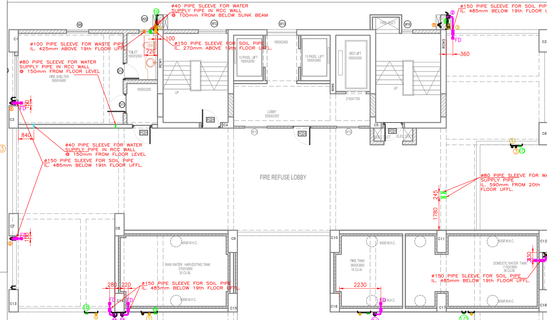
19TH FLOOR PLAN - TOILET DRAINAGE SCALE 1:20
