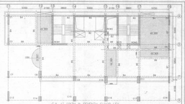
G.A. AT SIXTH & SEVENTH FLOOR LEV. UNO. ALL DIMS ARE IN METERS.
