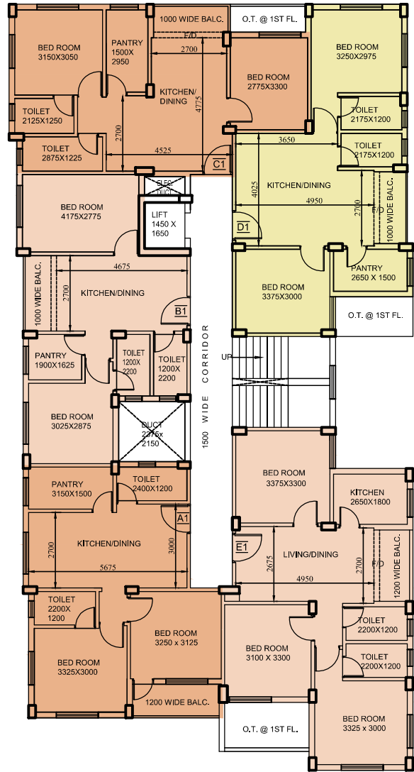
TYPICAL FLOOR PLAN (2nd,3rd & 4th floor)
