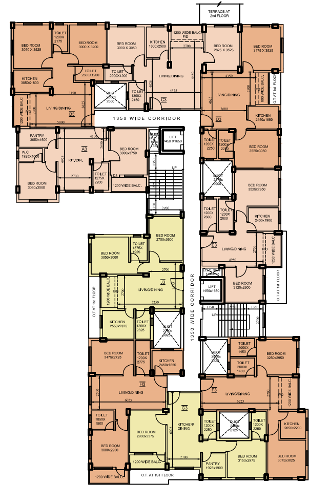
3rd - 4th FLOOR PLAN
