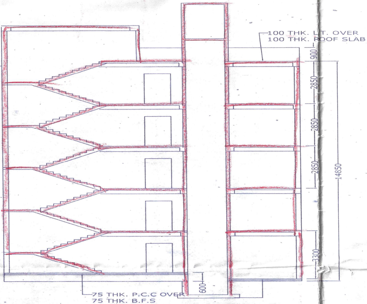
SECTION ON Y-Y1 BLOCK-B
