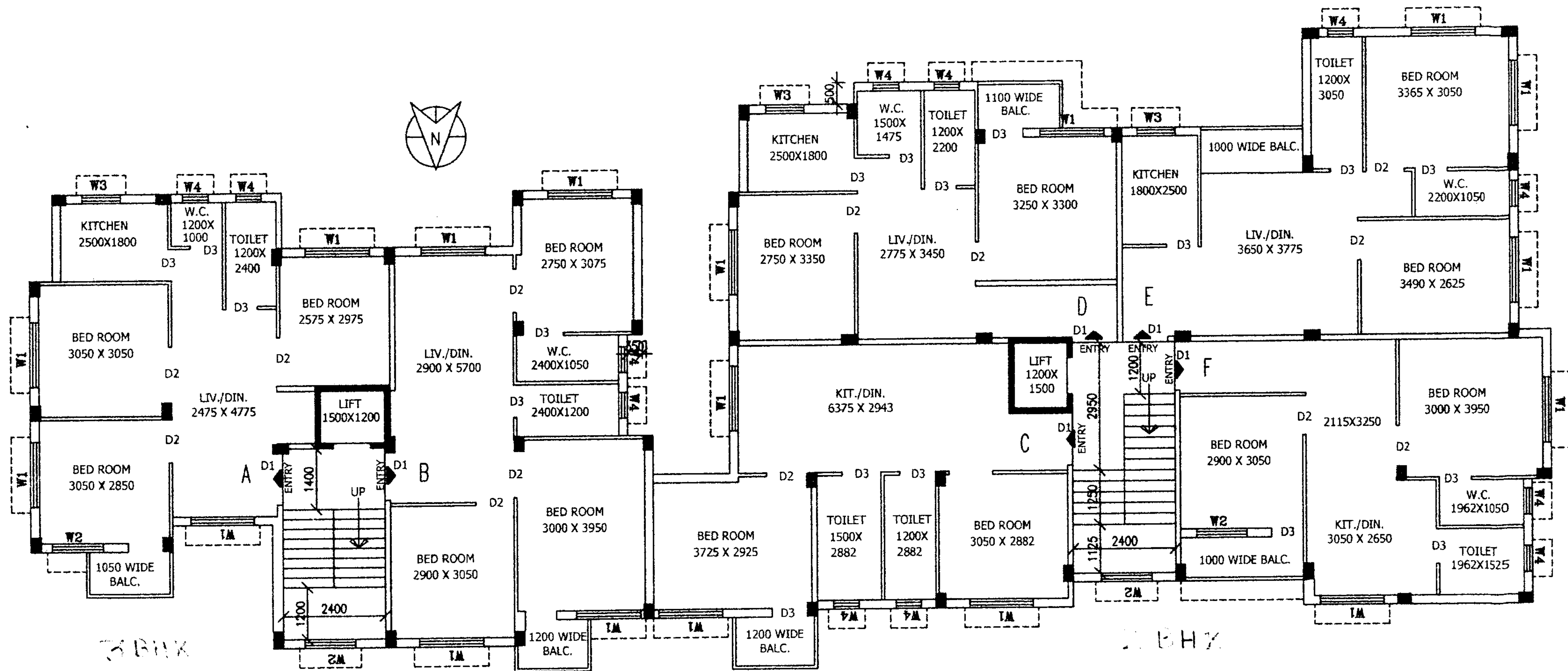
1ST, 2ND & 3RD FLOOR PLAN
