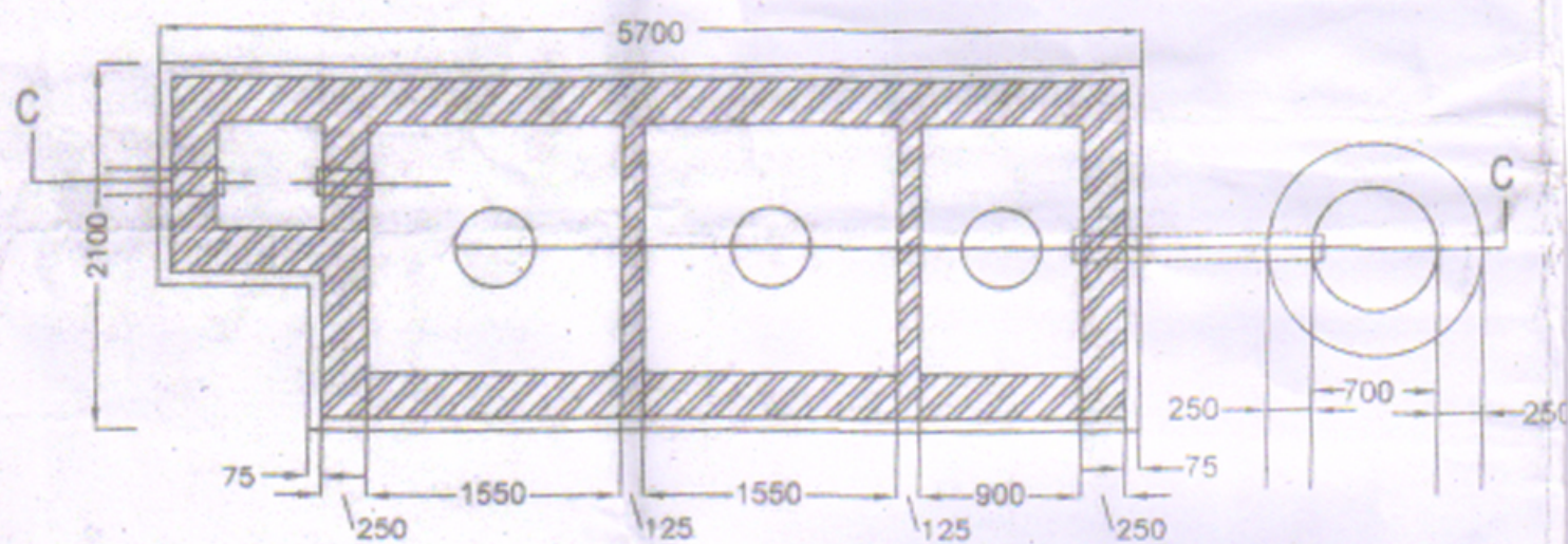
PLAN OF SEPTIC TANK & SOAK-PIT
