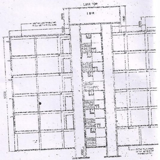
SECTION - X-X1
