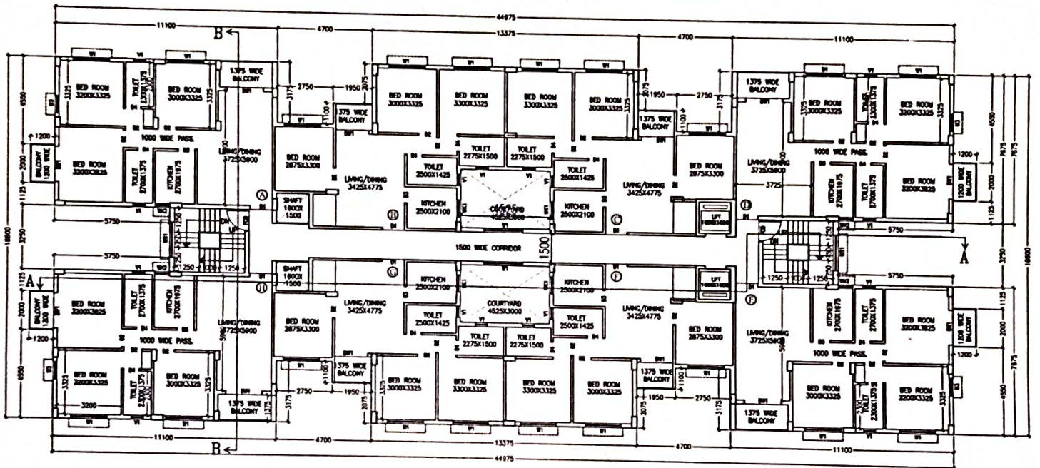
TYPICAL FLOOR PLAN (1ST TO 6TH FLOOR) BLOCK - 1
