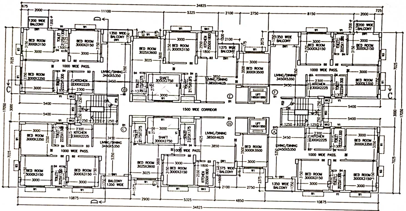
TYPICAL FLOOR PLAN (1ST TO 6TH FLOOR) BLOCK - 2
