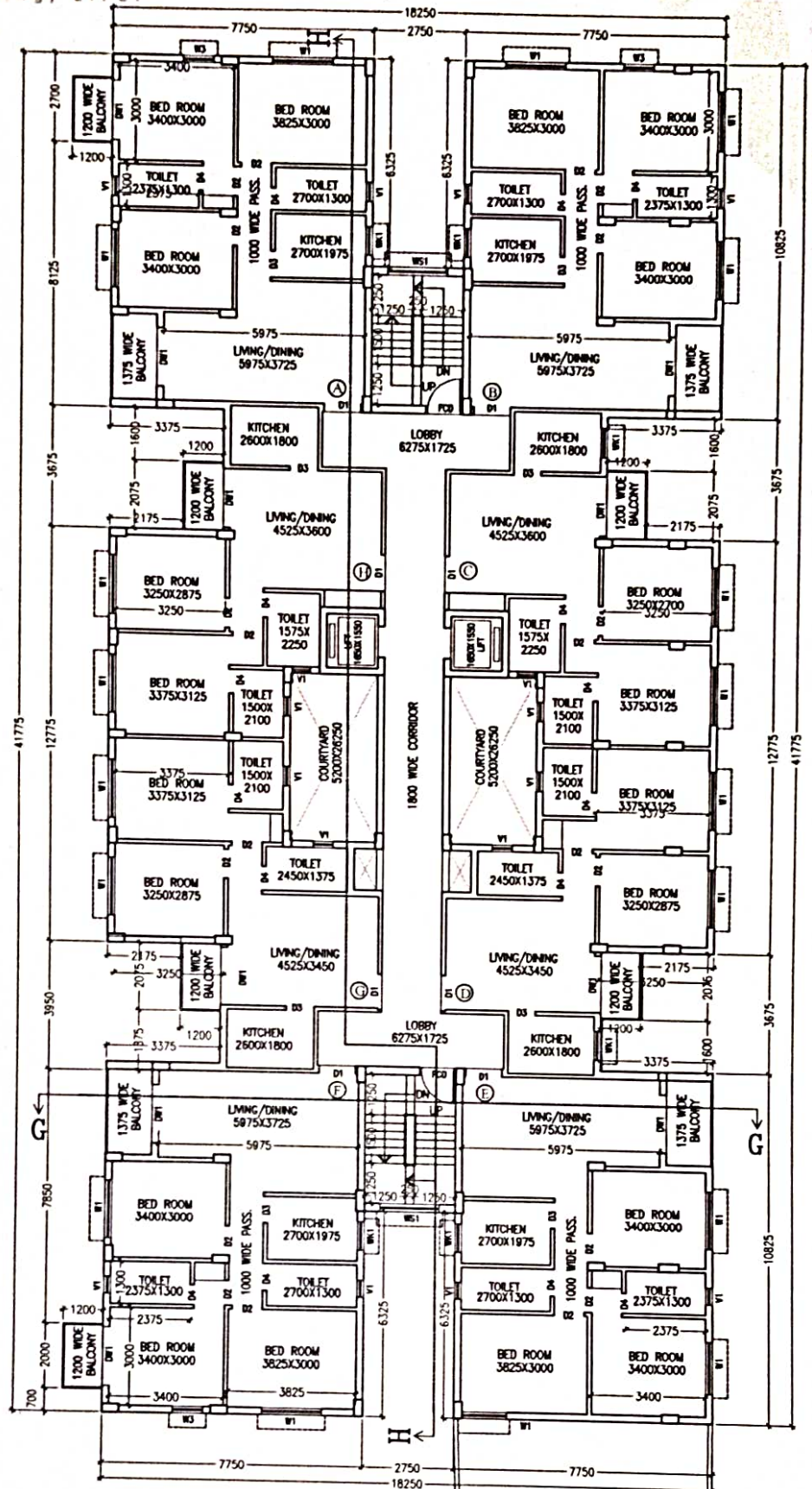
TYPICAL FLOOR PLAN (1ST TO 6TH FLOOR) ASPIRA LOHARUKA DEVELOPERS LLP
