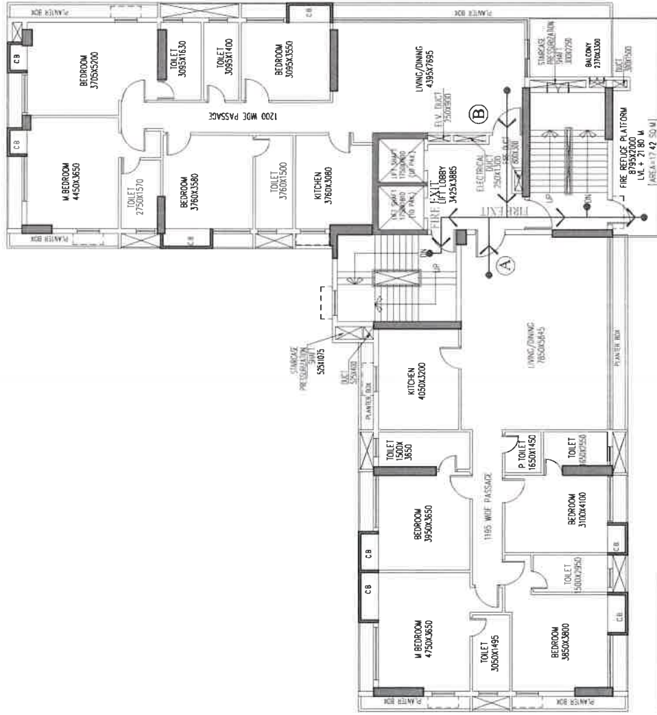
5TH FLOOR PLAN WITH FIRE REFUGE PLATFORM
