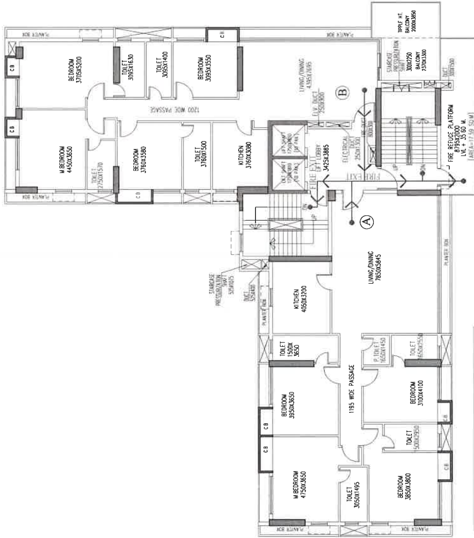
9TH FLOOR PLAN WITH FIRE REFUGE PLATFORM
