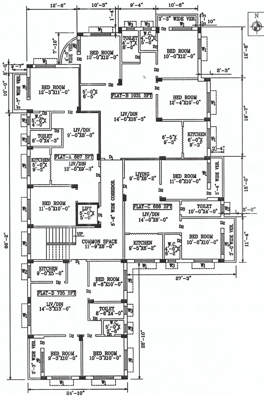
PROPOSED 1ST, 2ND, 3RD & 4TH FLOOR PLAN SCALE- 1:100 BLOCK-C
