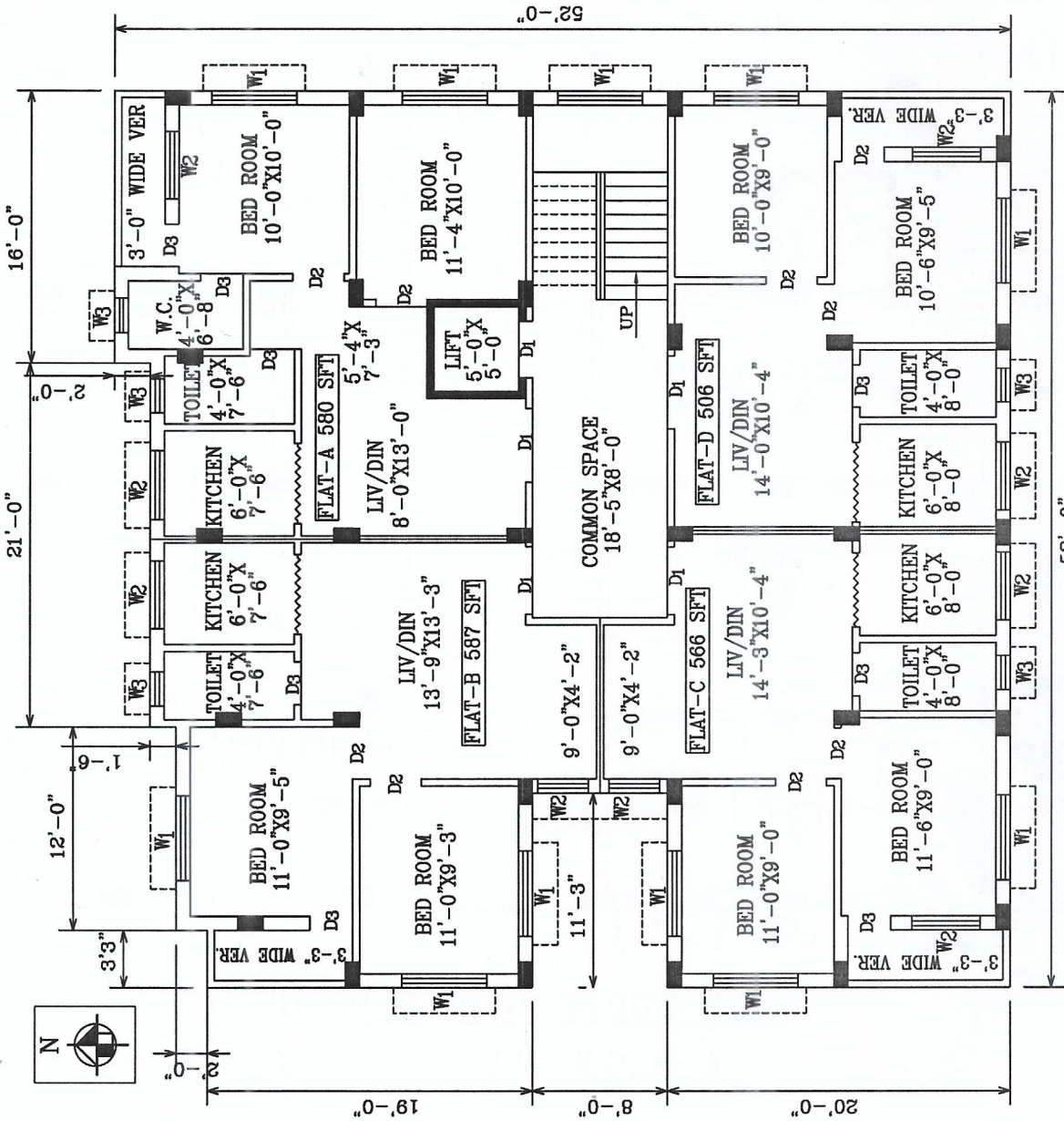
PROPOSED 1ST, 2ND, 3RD & 4TH FLOOR PLAN
