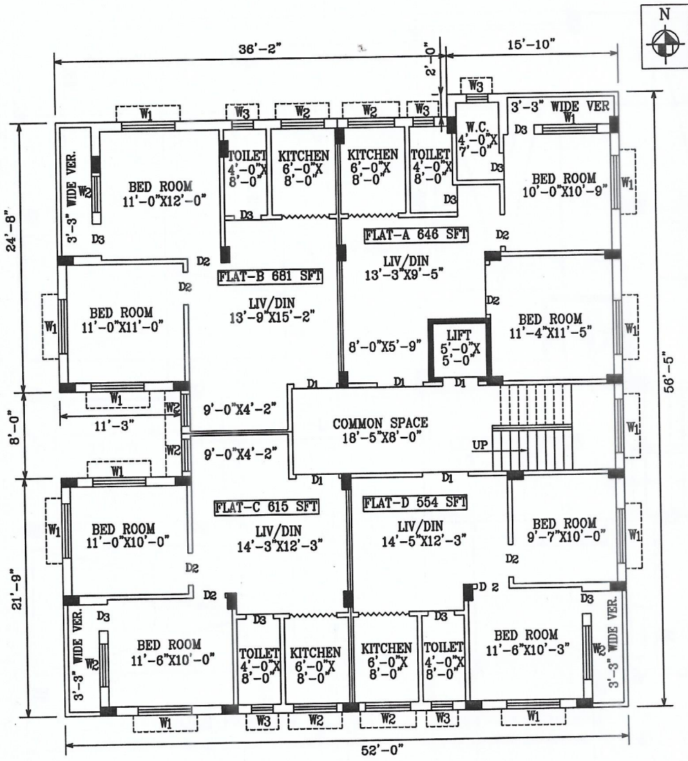
PROPOSED 1ST, 2ND, 3RD & 4TH FLOOR PLAN SCALE - 1:100 BLOCK-B
