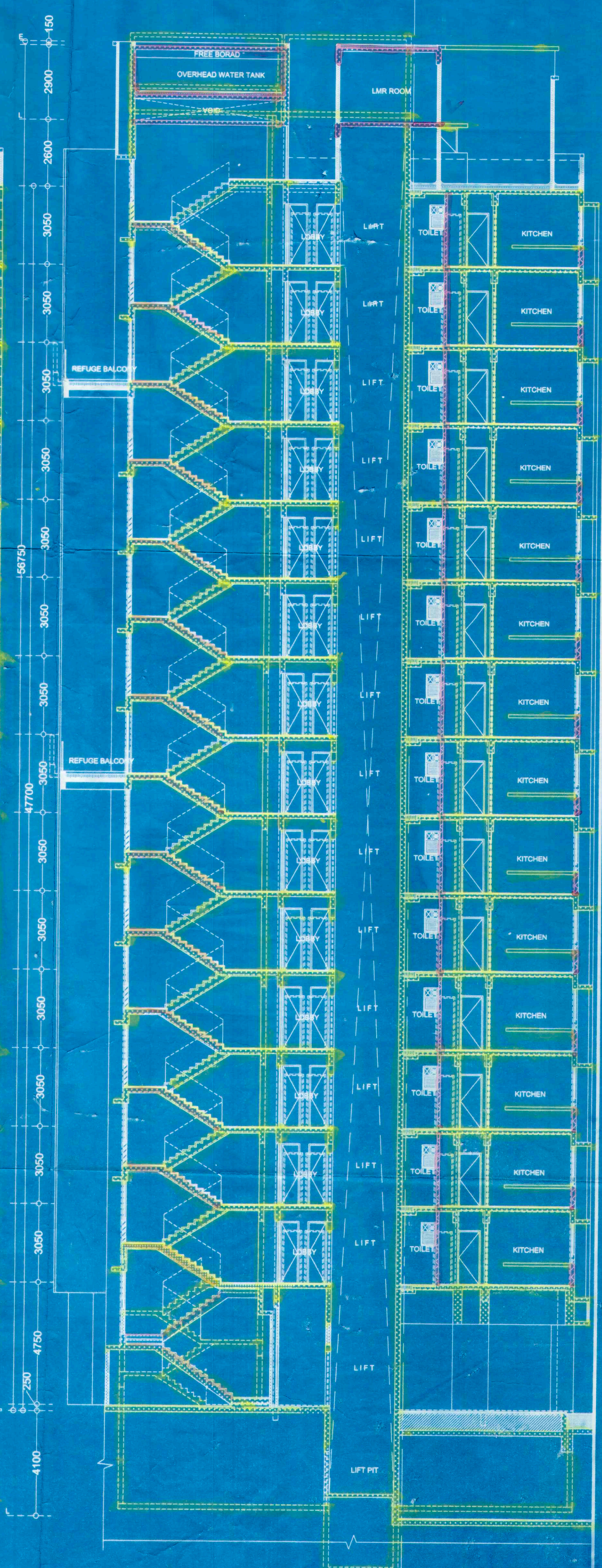
SECTION-BB SCALE- 1:100
