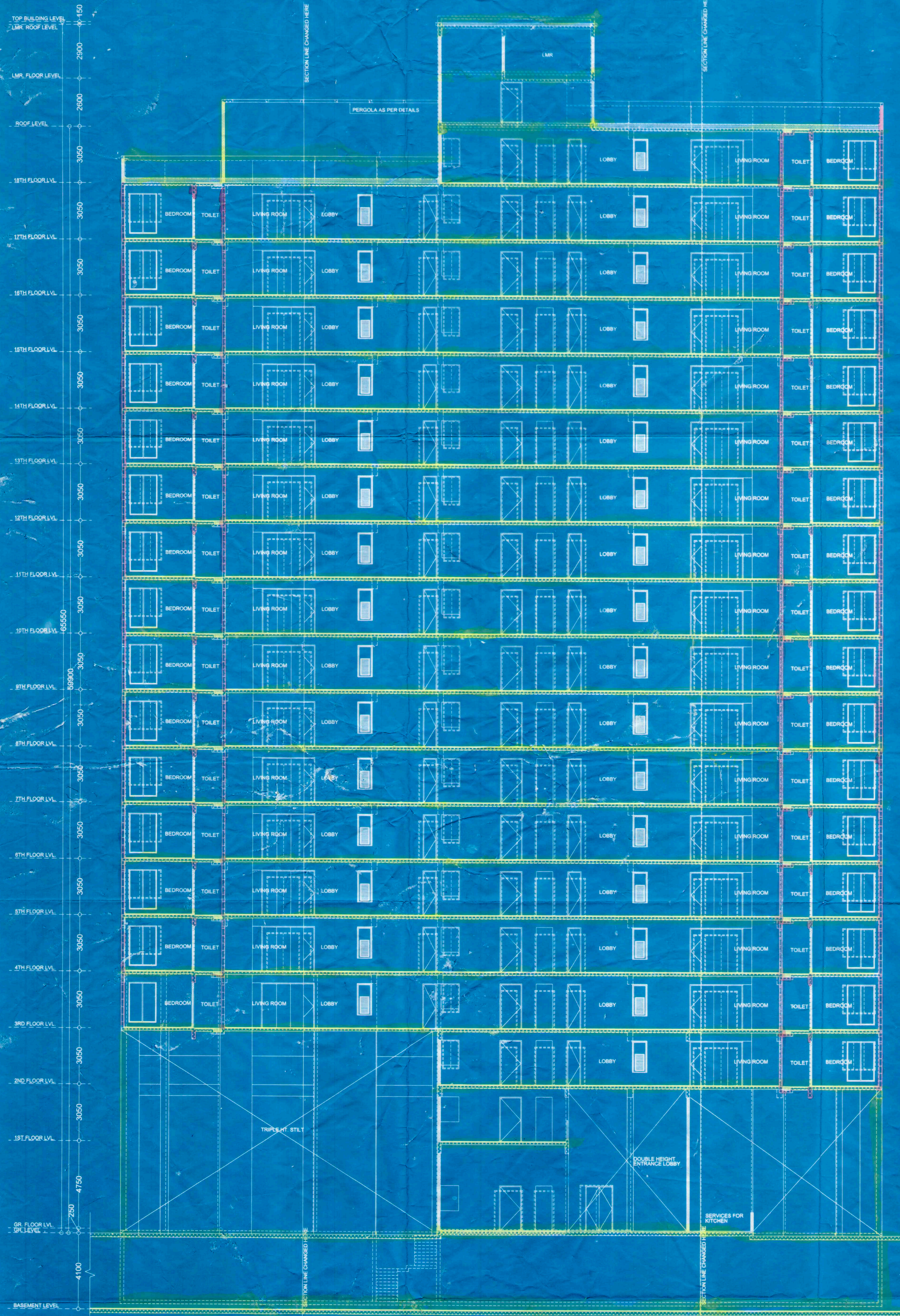
SECTION-GG SCALE- 1:100
