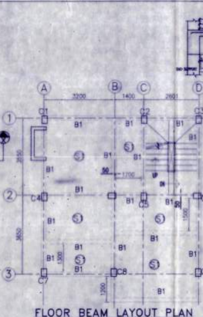
FLOOR BEAM LAYOUT PLAN SCALE 1:100
