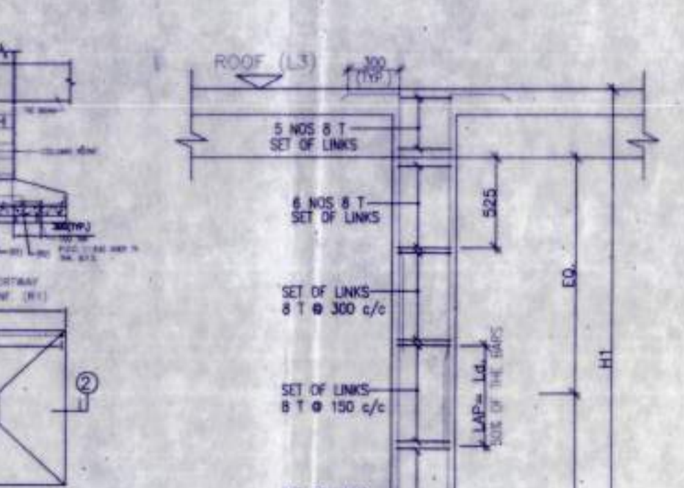
TYPICAL DETAIL OF COLUMN
