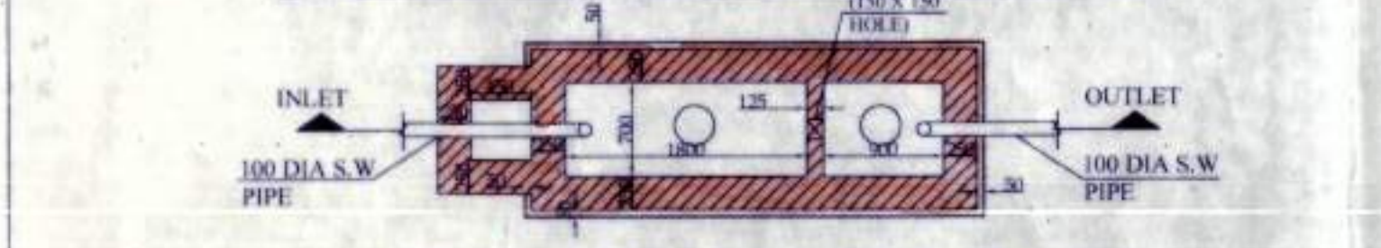
PLAN OF SEPTIC TANK (for 20 users)
