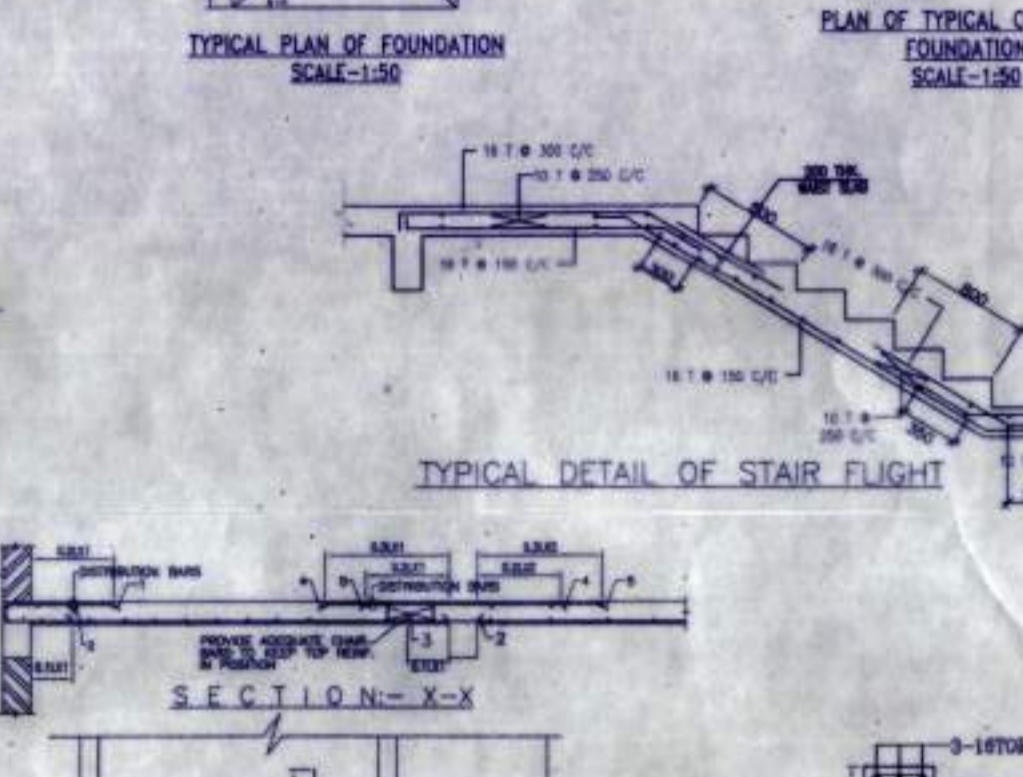
TYPICAL DETAIL OF STAIR FLIGHT
