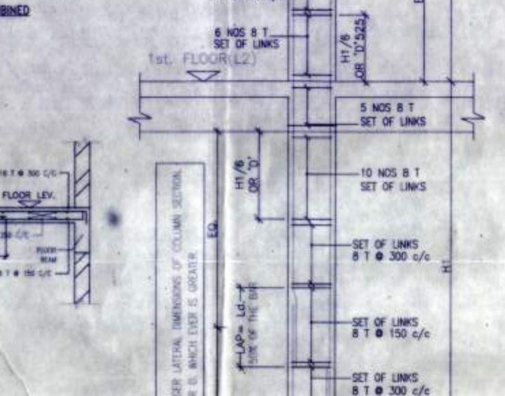
TYPICAL DETAIL OF COLUMN
