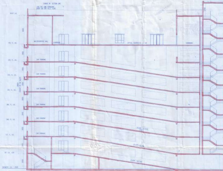
SECTION AT - H-H
