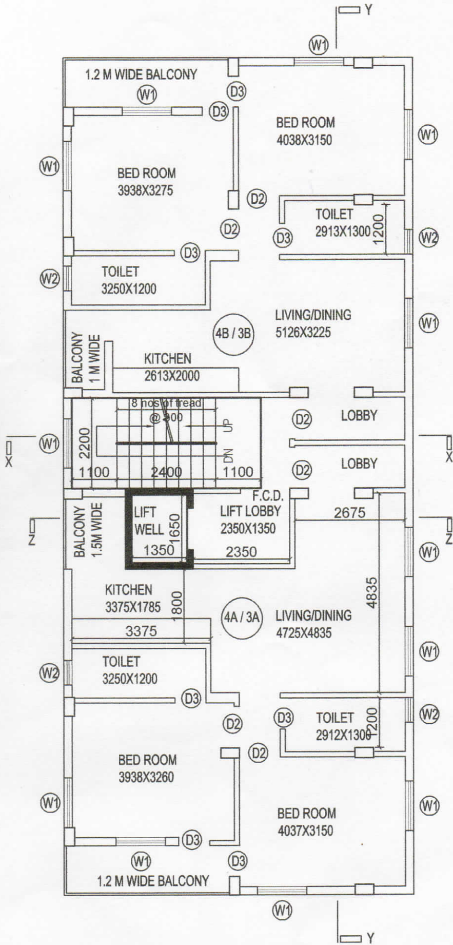
1ST, 2ND, 3RD, 4TH FLOOR PLAN (TYPICAL)
