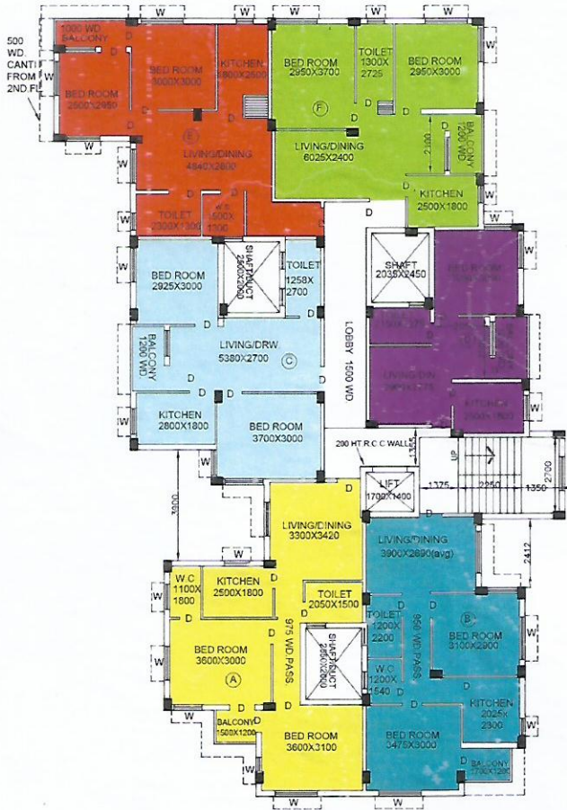
TYPICAL 1ST. FL. PLAN
