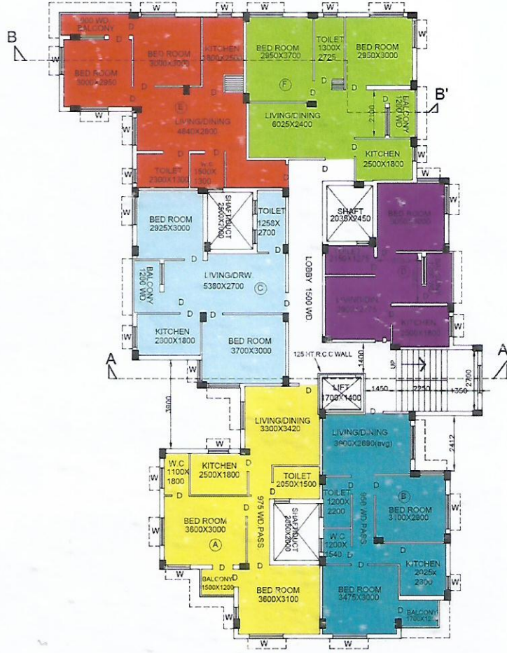
TYPICAL 2ND, 3RD, & 4TH, FL. PLAN
