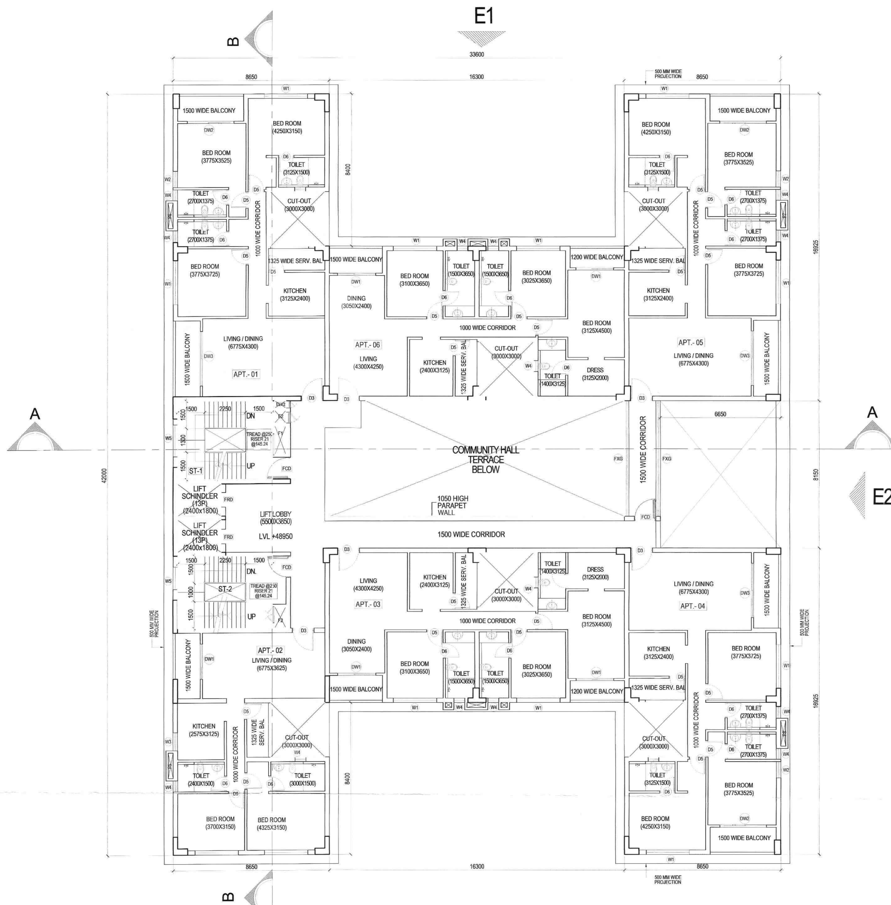
THIRTEENTH FLOOR PLAN SCALE: 1:100
