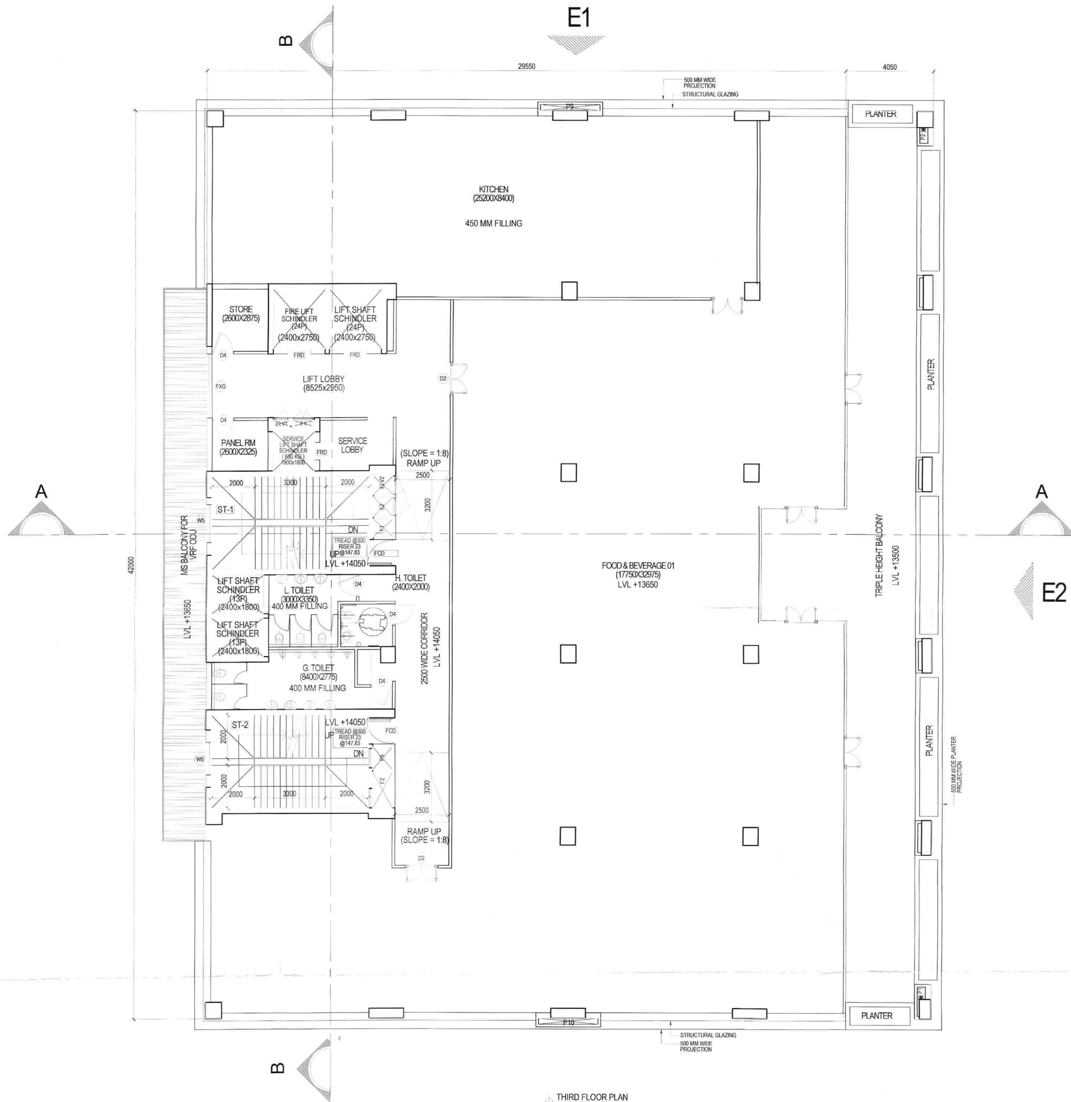
THIRD FLOOR PLAN SCALE: 1:100
