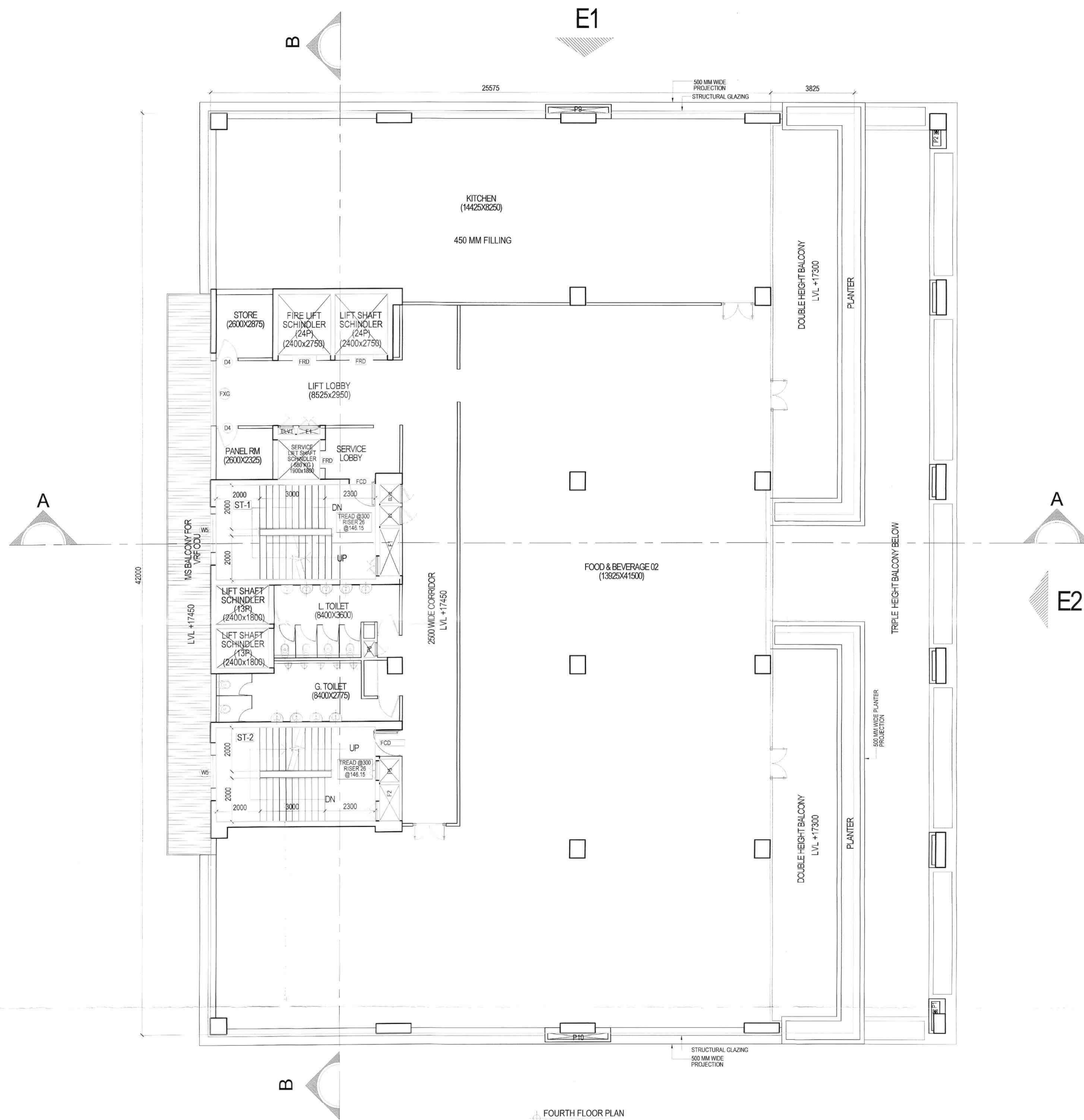
FOURTH FLOOR PLAN SCALE: 1:100
