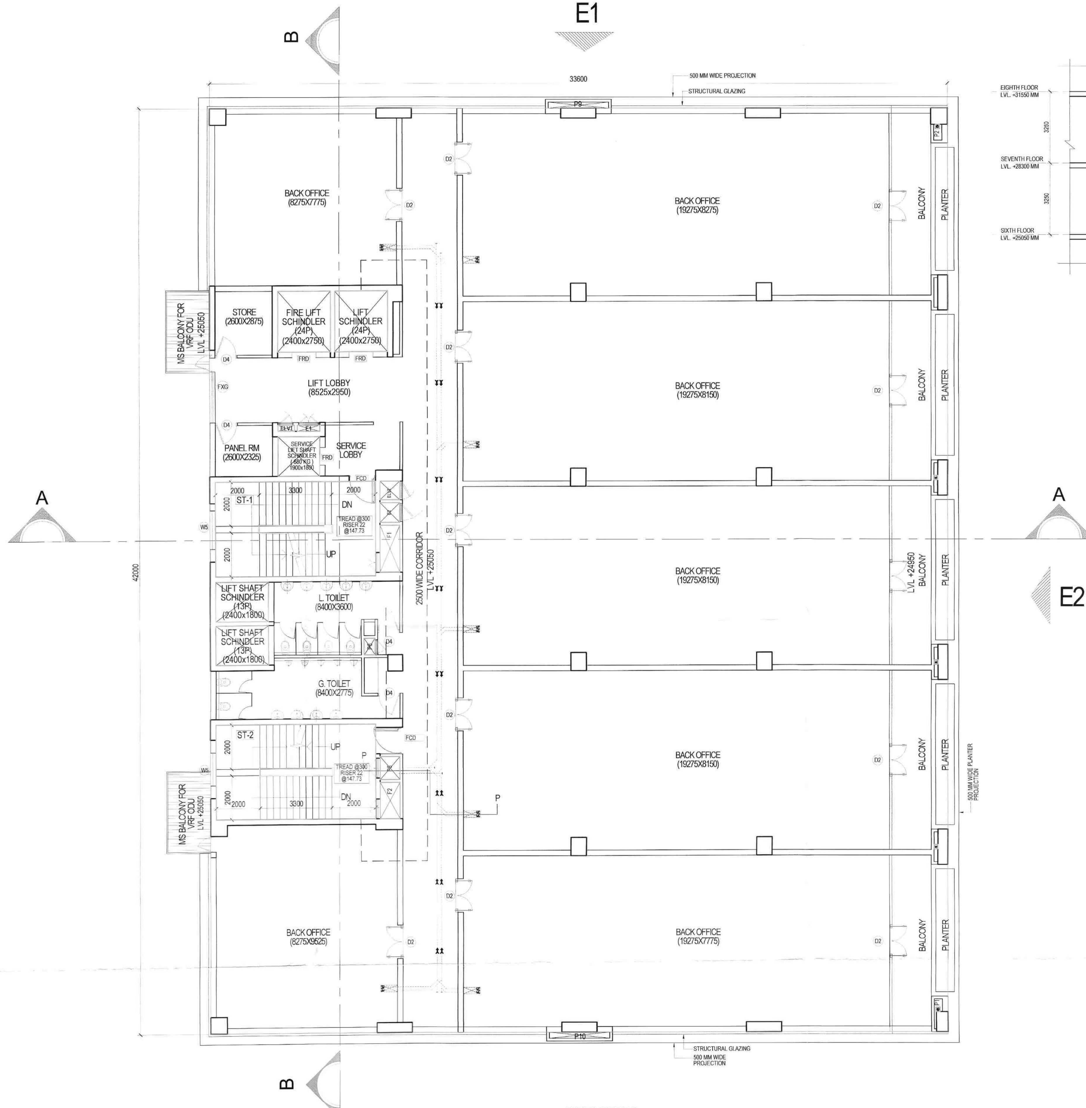
SIXTH FLOOR PLAN SCALE: 1:100
