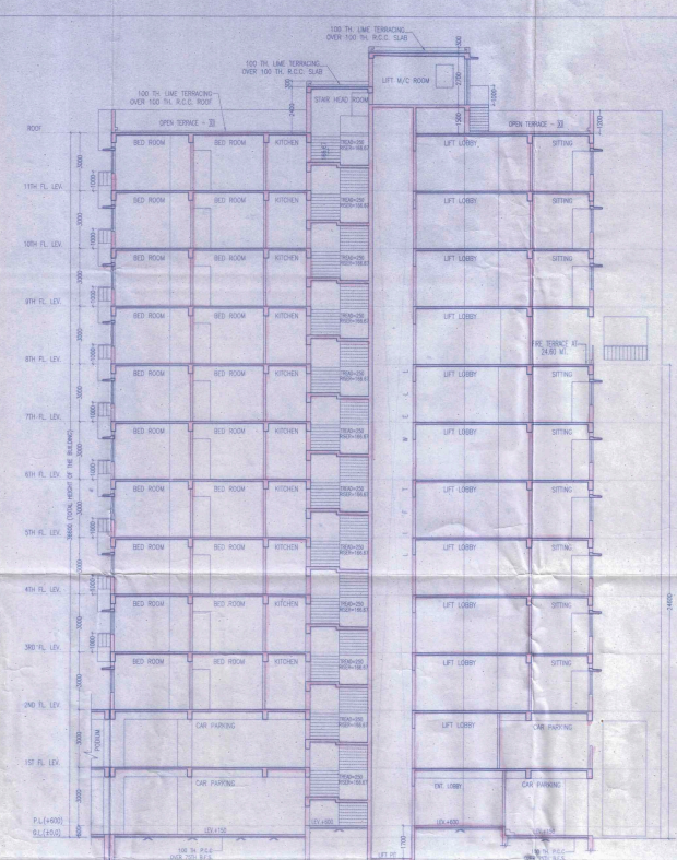
SECTION AT I-I BLOCK NO. - 7
