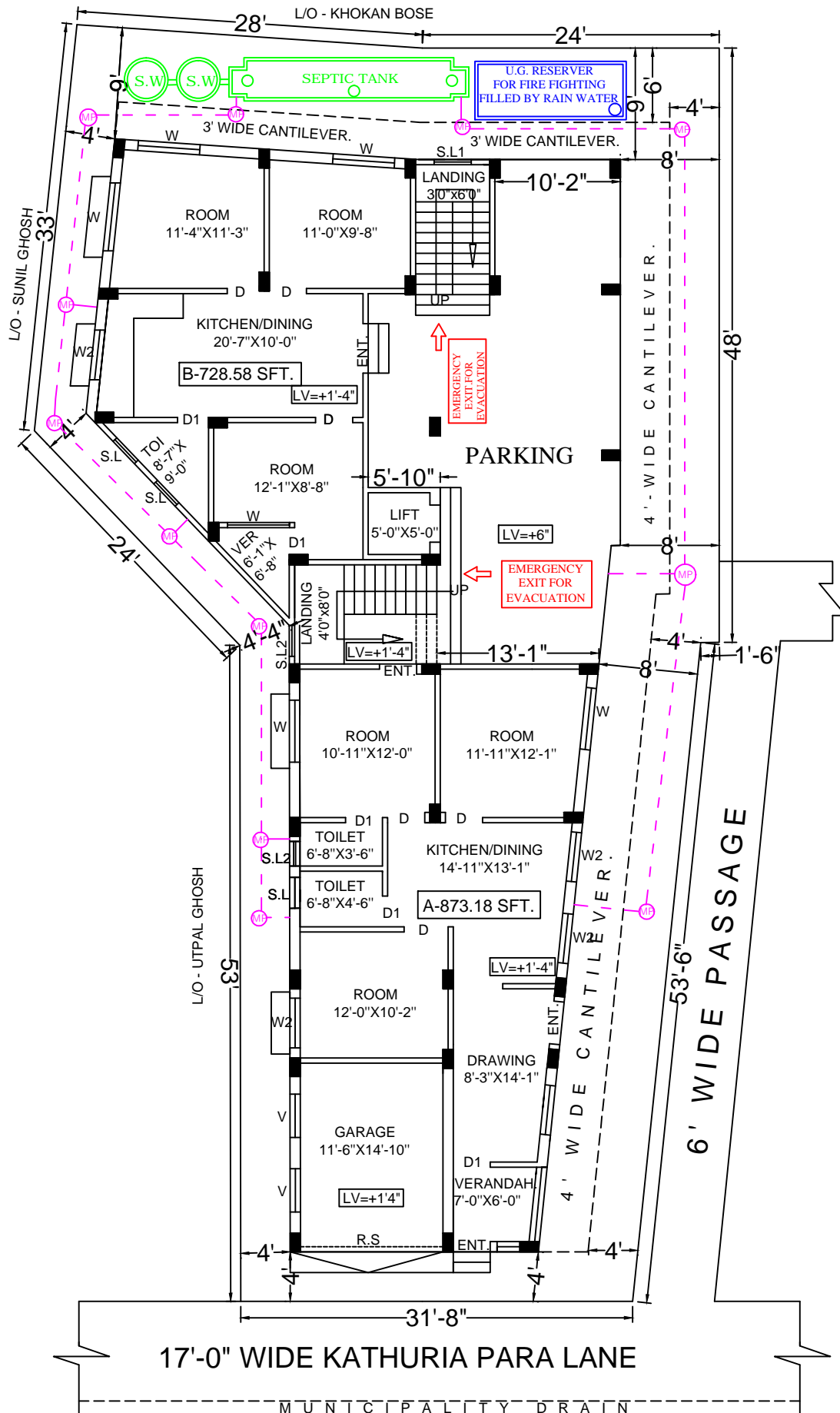
PROPOSED GROUND FLOOR PLAN WITH SITE PLAN SCALE - 1:96
