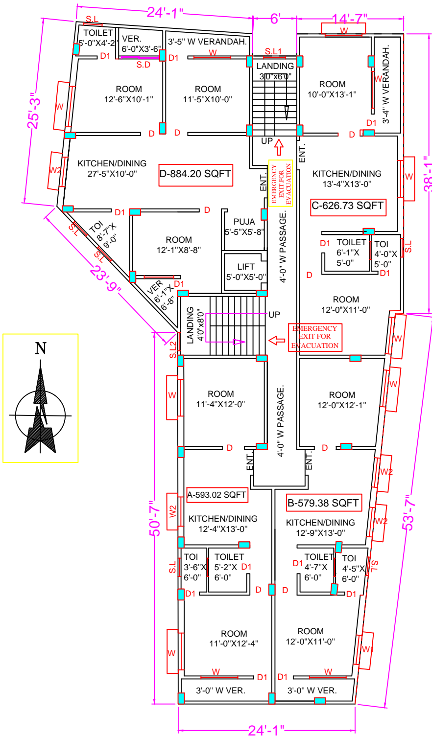
PROPOSED THIRD FLOOR PLAN SCALE - 1:96
