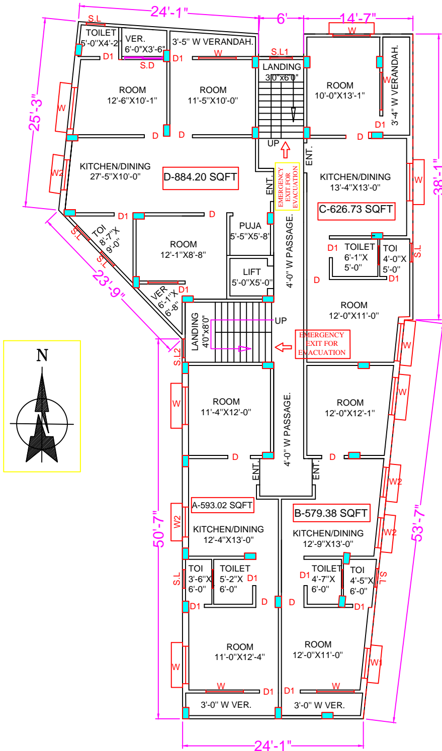
PROPOSED FIRST FLOOR PLAN SCALE - 1:96
