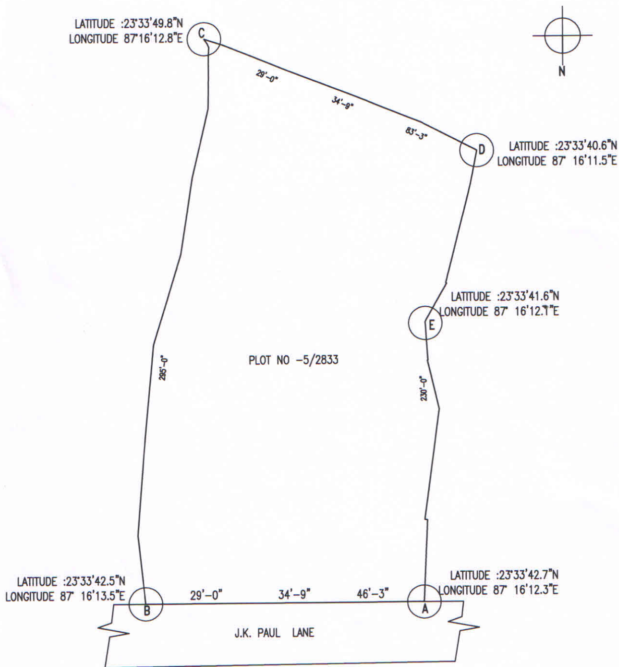
SITE PLAN
