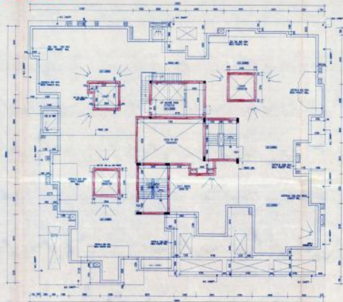
ROOF PLAN (BLOCK-A)
