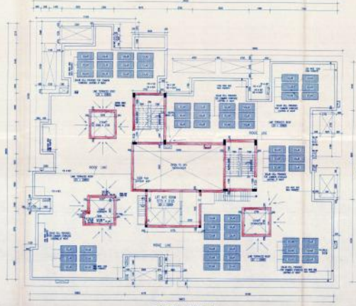
ROOF PLAN (BLOCK-B)
