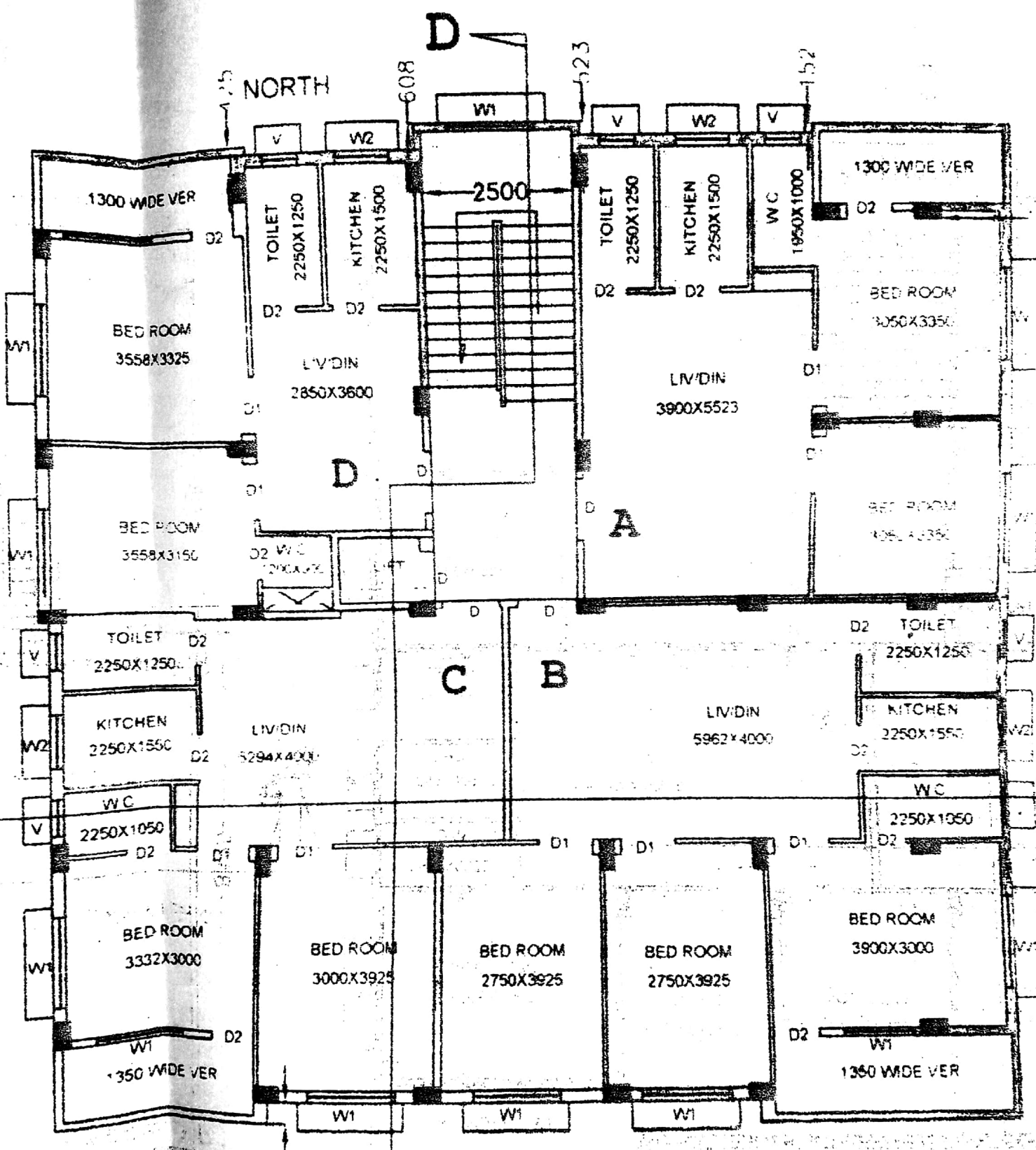
1ST TO 3RD FLOOR PLAN
