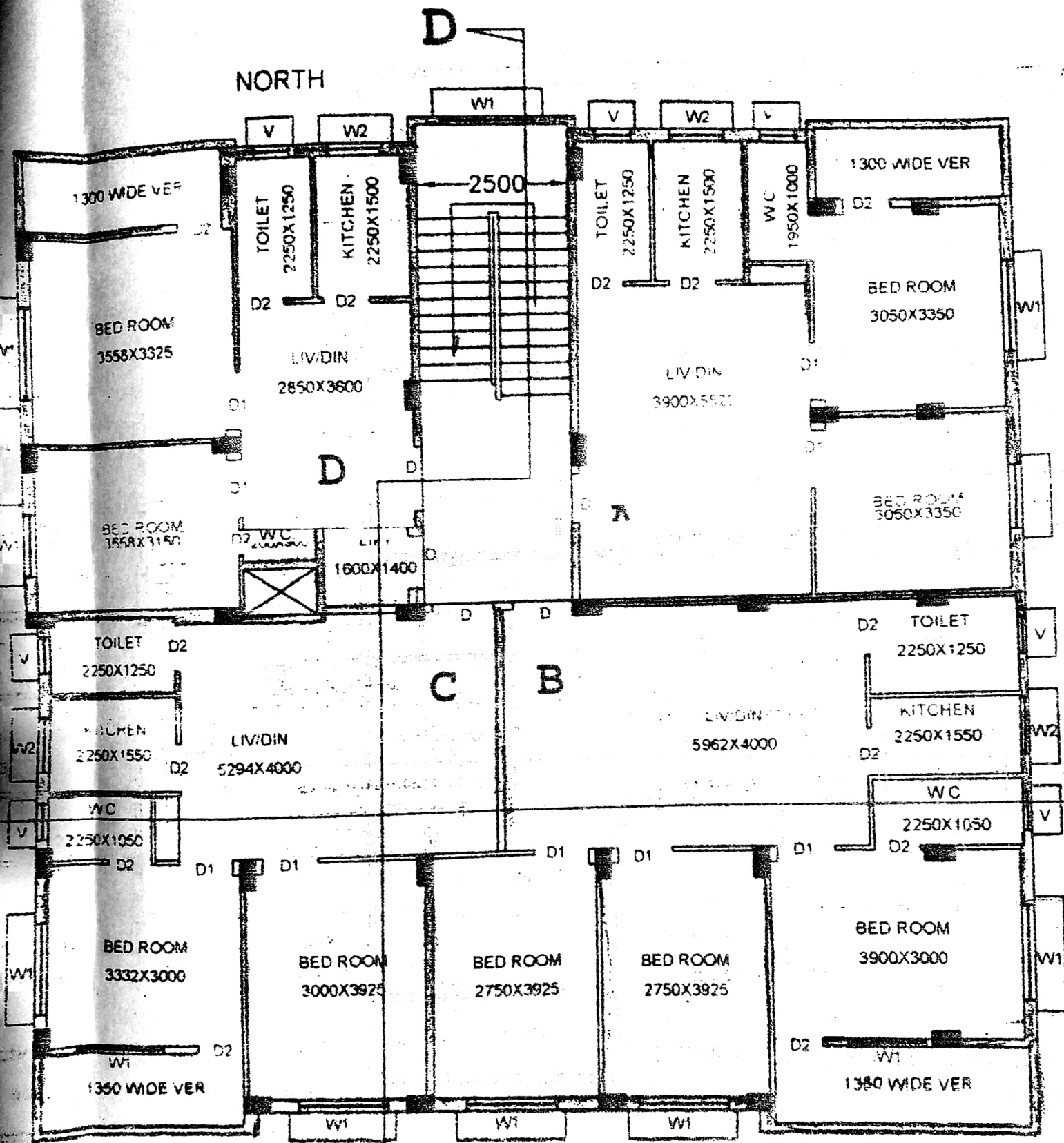
4TH FLOOR PLAN
