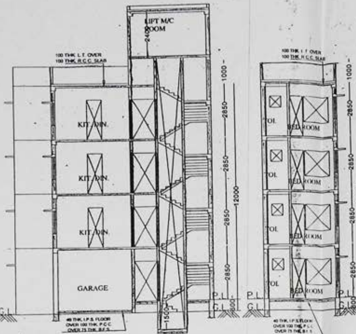
SECTION AT:- F-F
