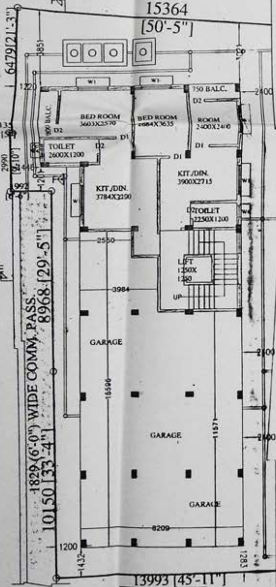
BLOCK-C GROUND FLOOR PLAN
