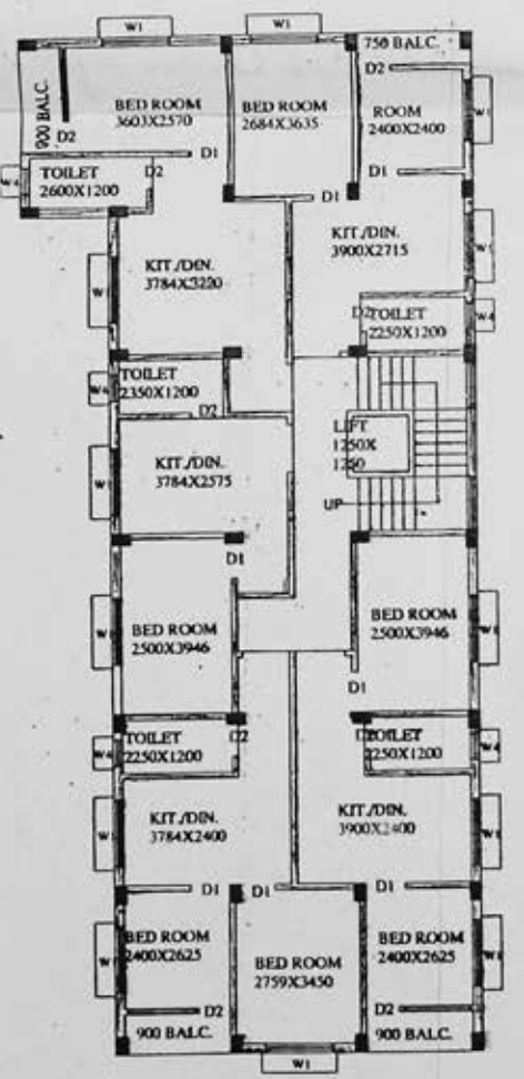
1ST, 2ND, 3RD FLOOR PLAN
