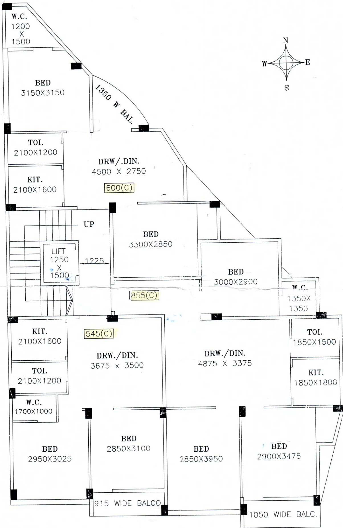
PROPOSED 1ST., 2ND. & 3RD. FLOOR PLAN
