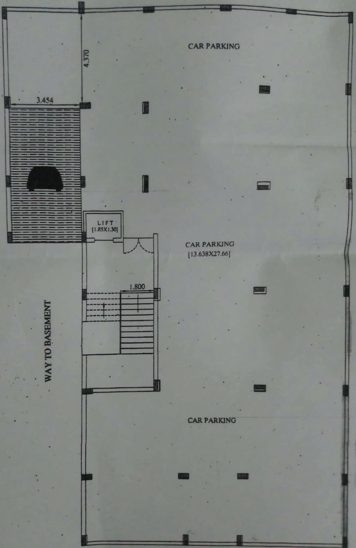
BASEMENT PLAN
