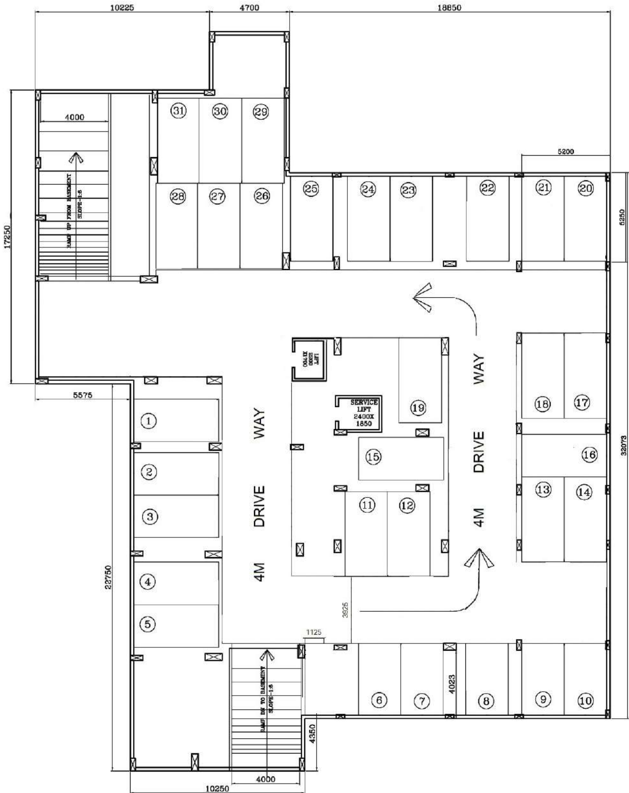
BASEMENT PLAN
