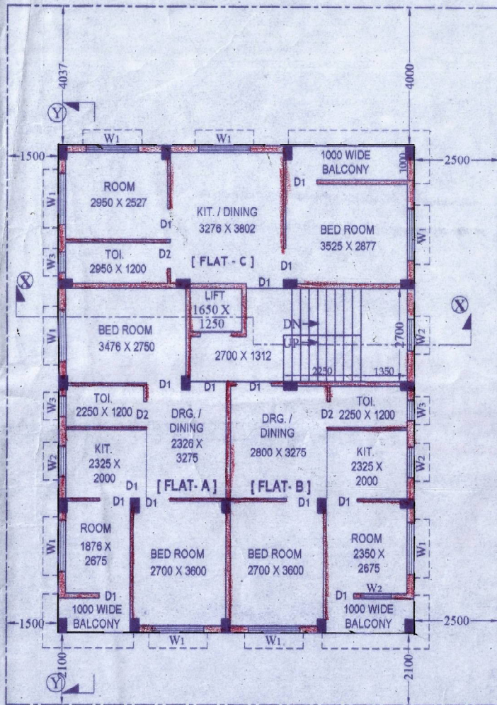
TYPICAL FLOOR PLAN (FIRST, SECOND, THIRD & FOURTH)
