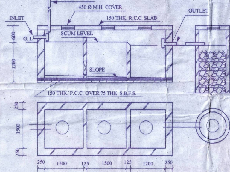
DETL. OF SEPTICTANK & SOAK PIT (FOR 50 USER)
