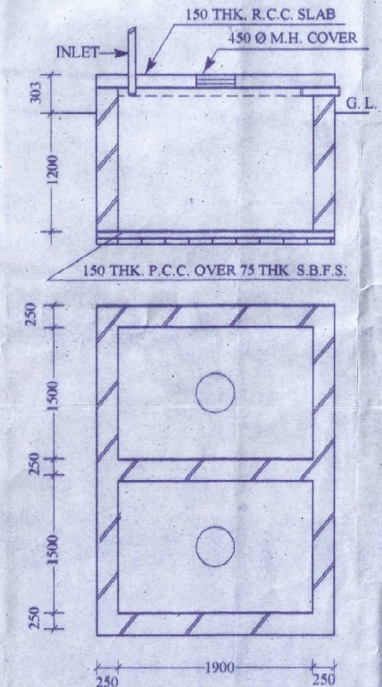
DETL. OF UNDER GROUND WATER RESERVIOR(U.G.R.)
