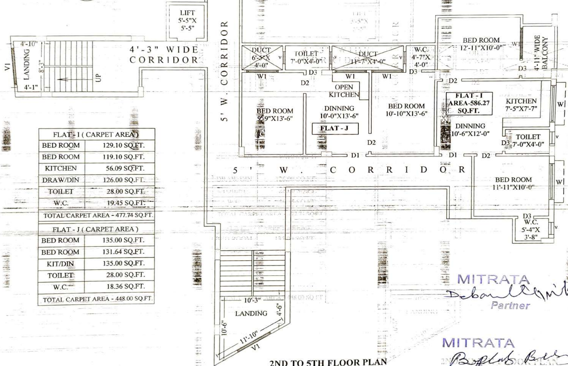
2ND TO 5TH FLOOR PLAN FLAT - I & FLAT - J SCALE - 1:96
