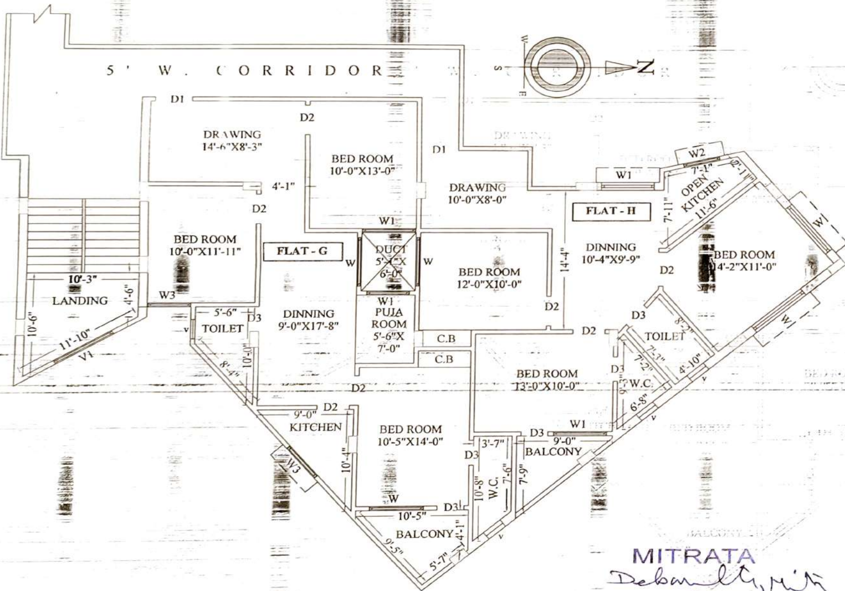
2ND TO 5TH FLOOR PLAN FLAT - G & FLAT - H SCALE - 1:96
